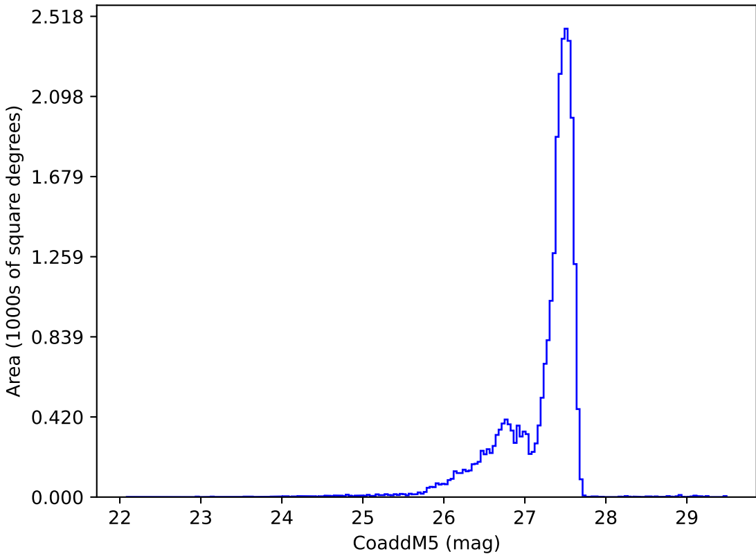
early_u_fpextra4.0_v3.4_10yrs : CoaddM5
