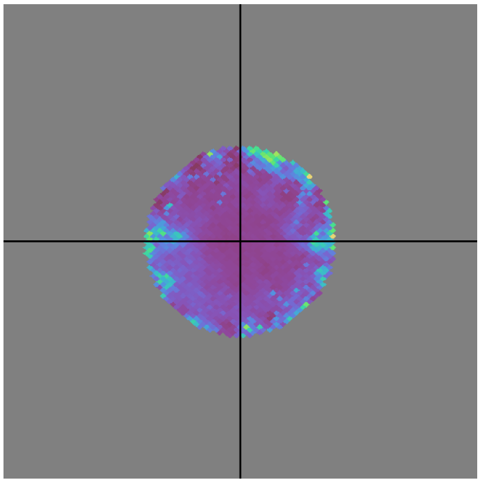
early_u_fpextra4.0_v3.4_10yrs DD: COSMOS u band: Structure Function Uncert
