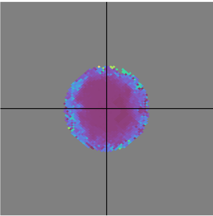
early_u_fpextra4.0_v3.4_10yrs DD: COSMOS i band: Structure Function Uncert
