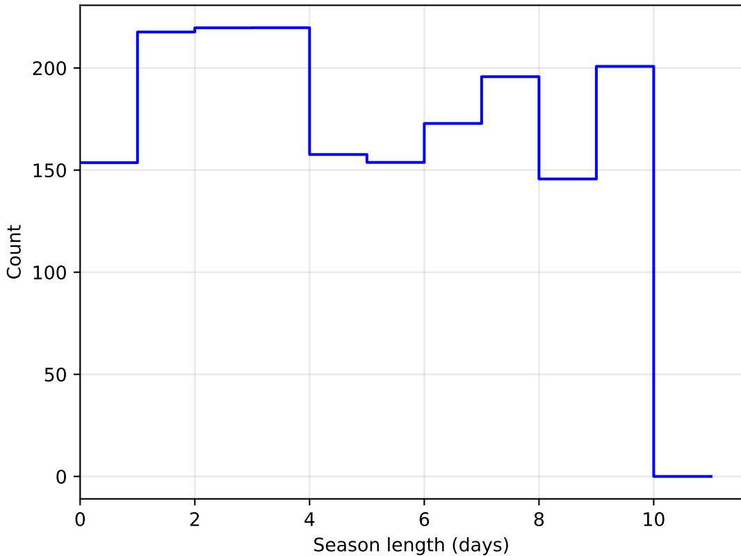
early_u_fpextra4.0_v3.4_10yrs DD:WFD all bands: SeasonLength
