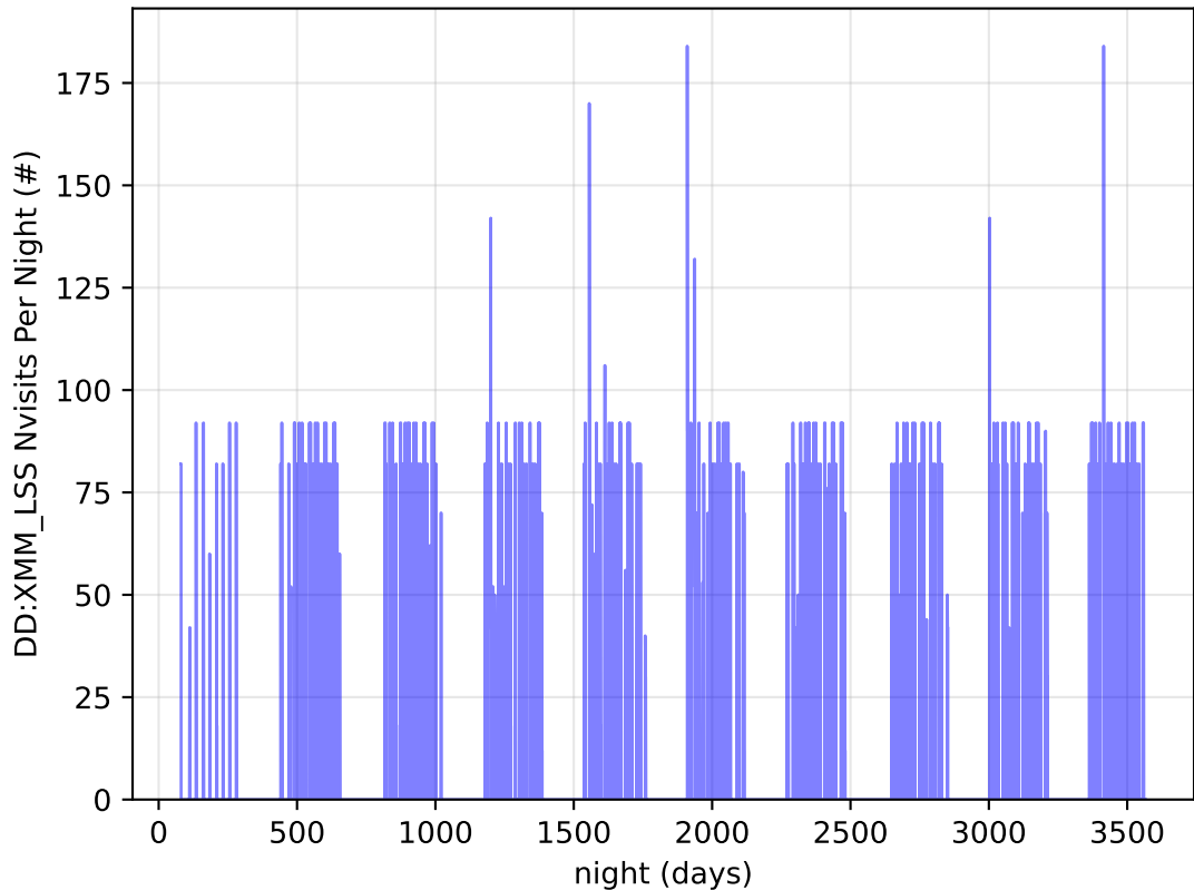
early_u_fpextra4.0_v3.4_10yrs all bands: DD:XMM_LSS Nvisits Per Night
