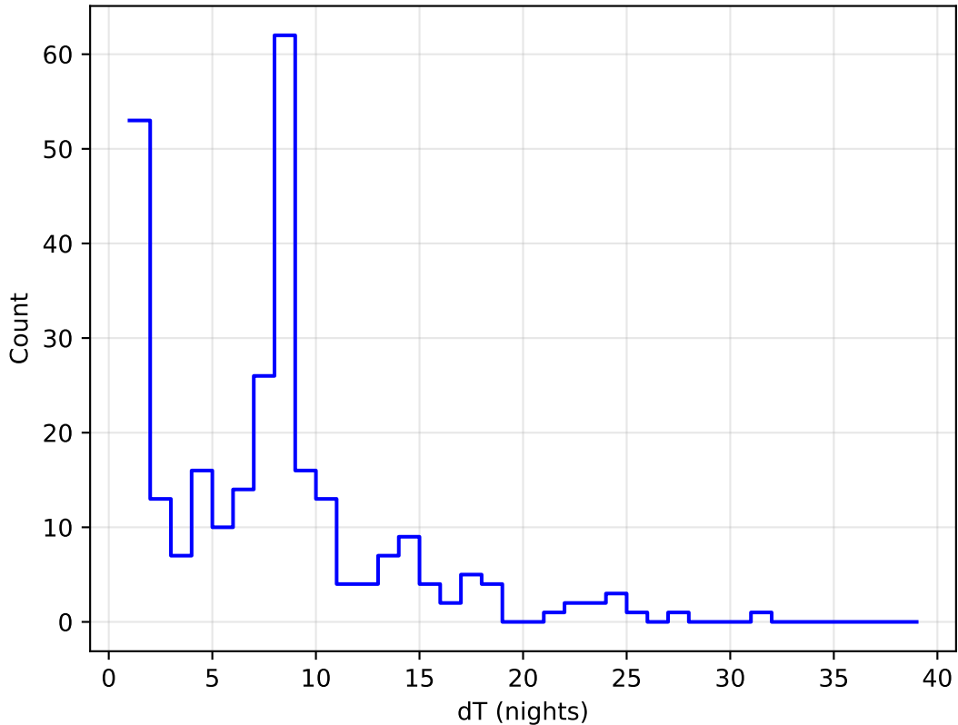
early_u_fpextra4.0_v3.4_10yrs all bands: DD:XMM_LSS Delta Nights Histogram
