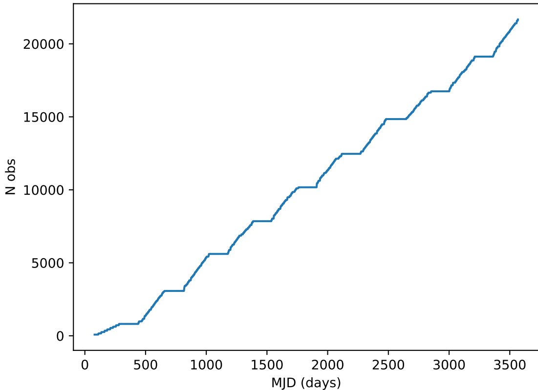
early_u_fpextra4.0_v3.4_10yrs all bands: DD:XMM_LSS Cumulative NVisits
