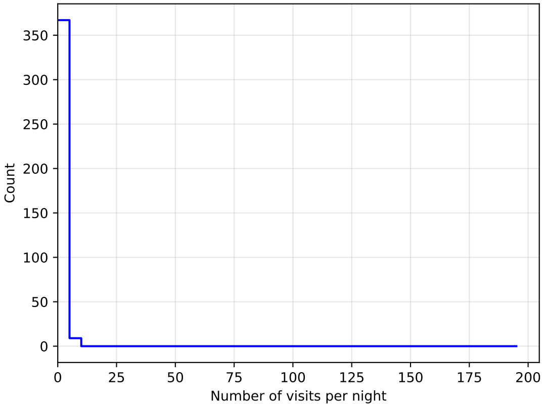
early_u_fpextra4.0_v3.4_10yrs all bands: DD:WFD NVisitsPerNight
