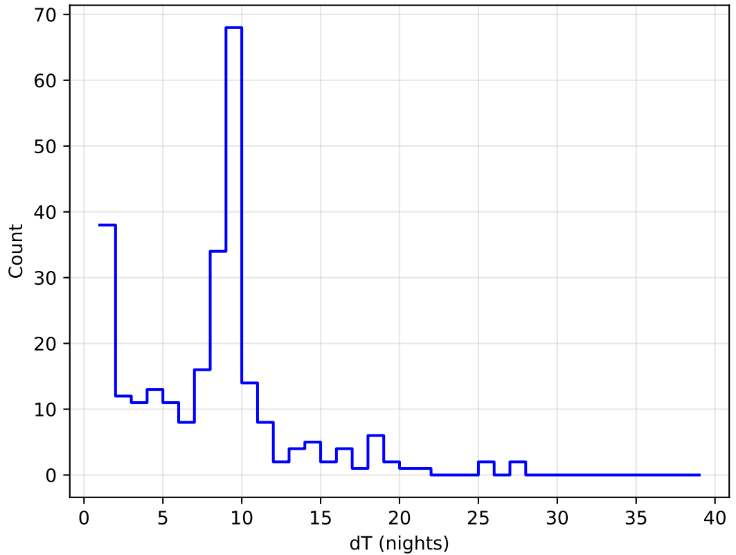
early_u_fpextra4.0_v3.4_10yrs all bands: DD:ELAISS1 Delta Nights Histogram
