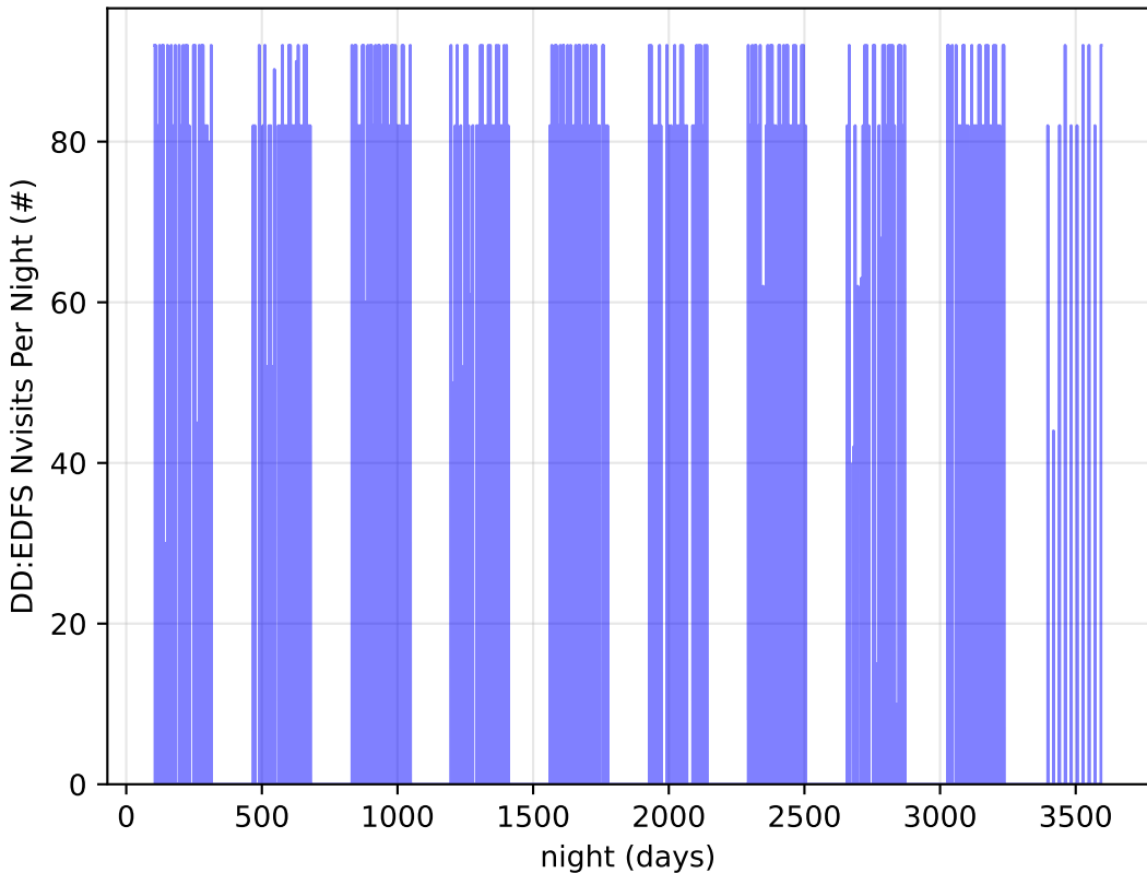
early_u_fpextra4.0_v3.4_10yrs all bands: DD:EDFS Nvisits Per Night
