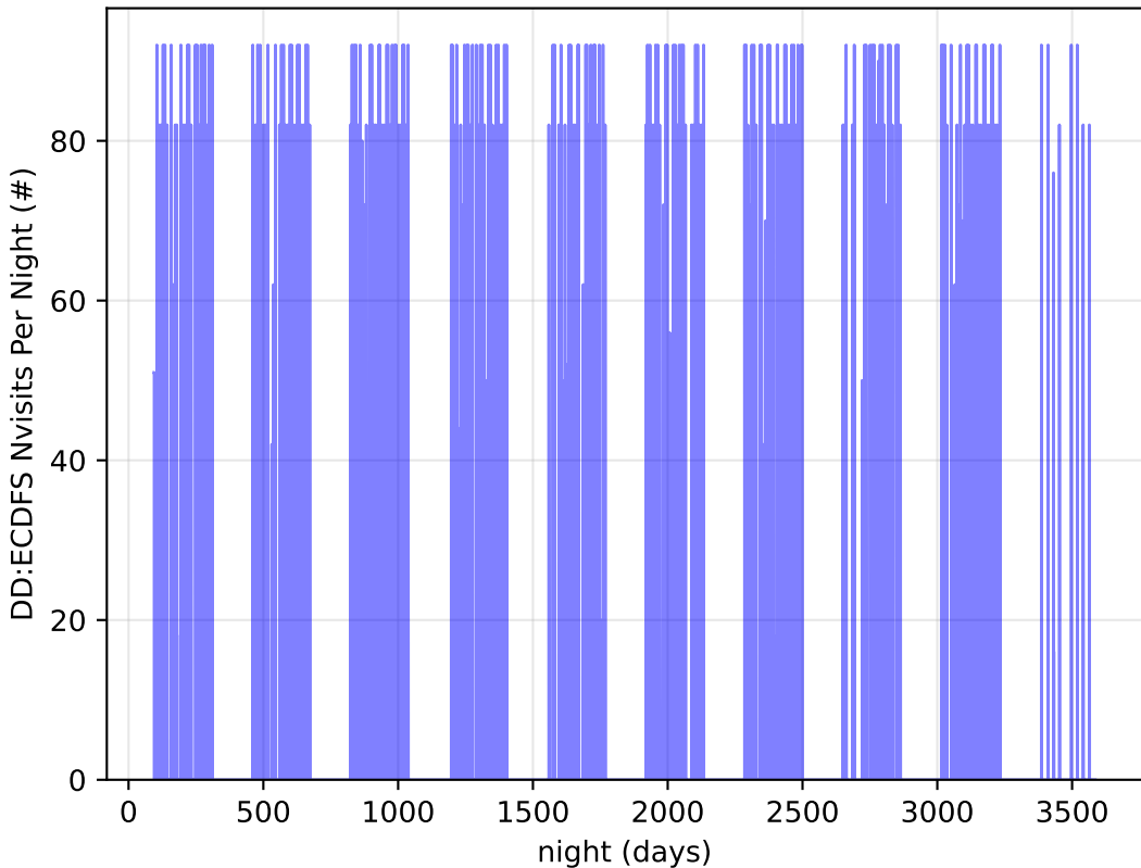
early_u_fpextra4.0_v3.4_10yrs all bands: DD:ECDFS Nvisits Per Night
