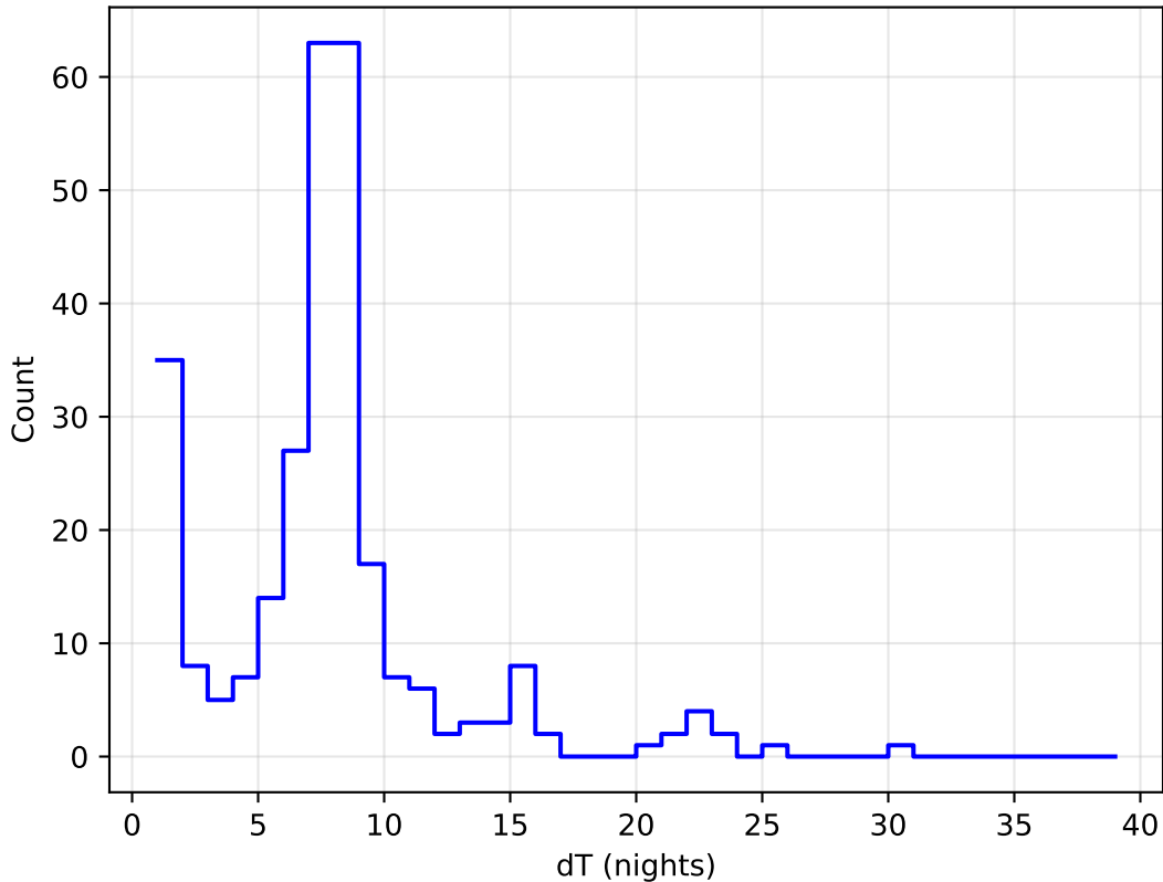
early_u_fpextra4.0_v3.4_10yrs all bands: DD:ECDFS Delta Nights Histogram
