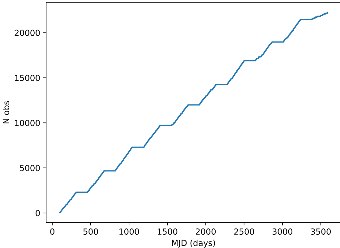
early_u_fpextra4.0_v3.4_10yrs all bands: DD:ECDFS Cumulative NVisits
