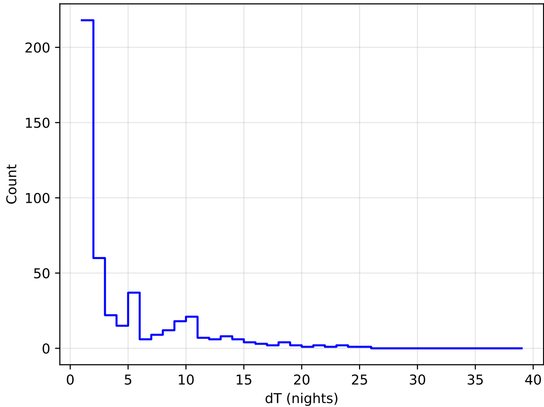
early_u_fpextra4.0_v3.4_10yrs all bands: DD: COSMOS Delta Nights Histogram
