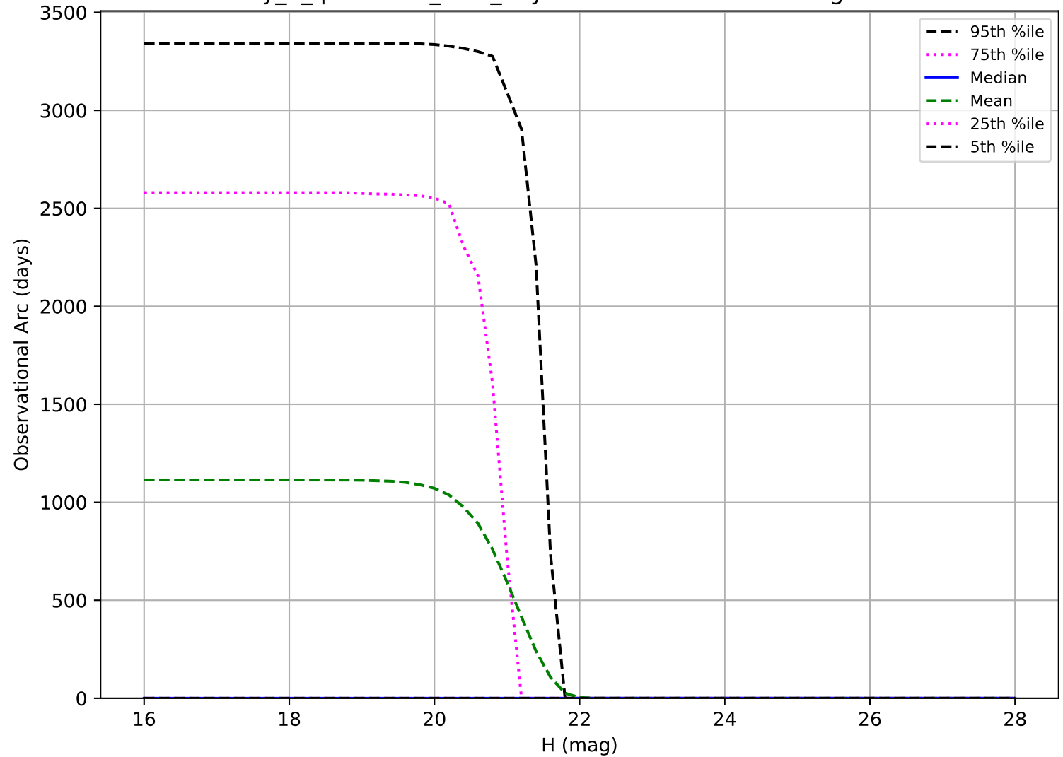
early_u_fpextra3.0_v3.4_10yrs: Observational Arc Length Vatra
