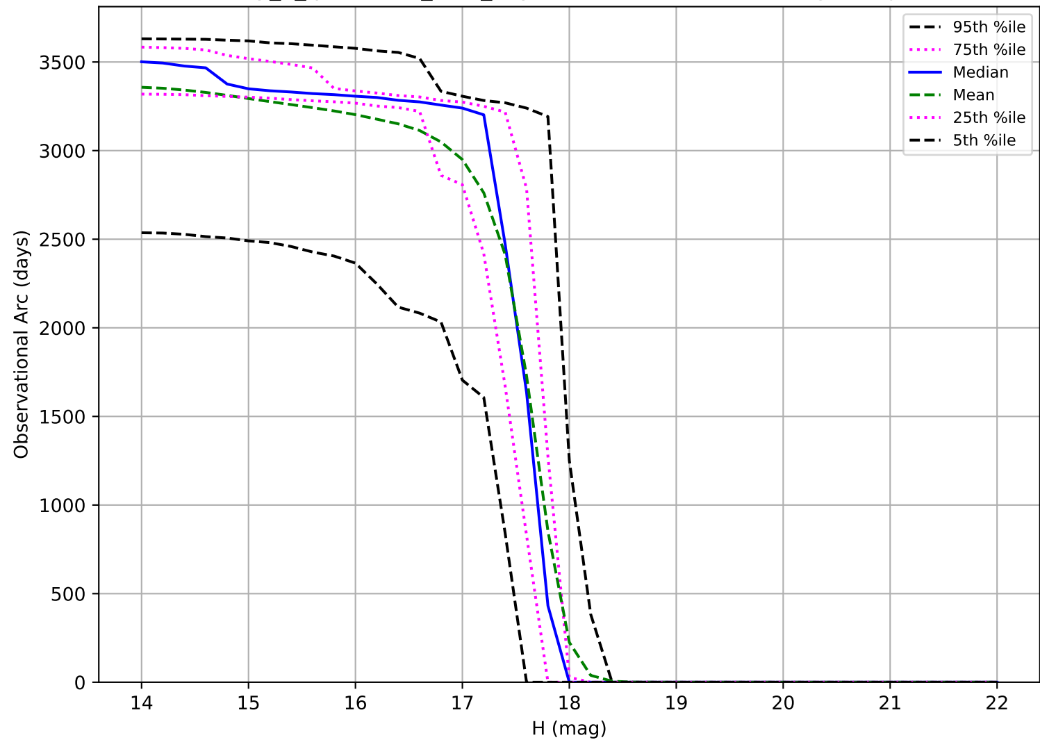
early_u_fpextra3.0_v3.4_10yrs: Observational Arc Length Trojan
