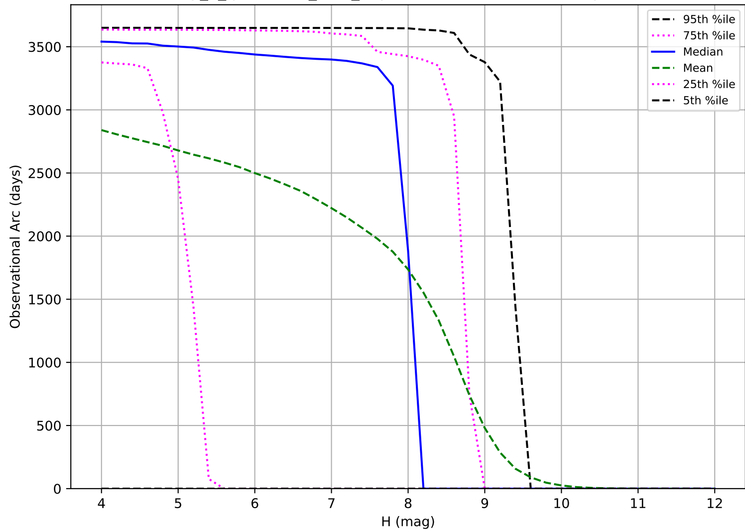
early_u_fpextra3.0_v3.4_10yrs: Observational Arc Length TNO
