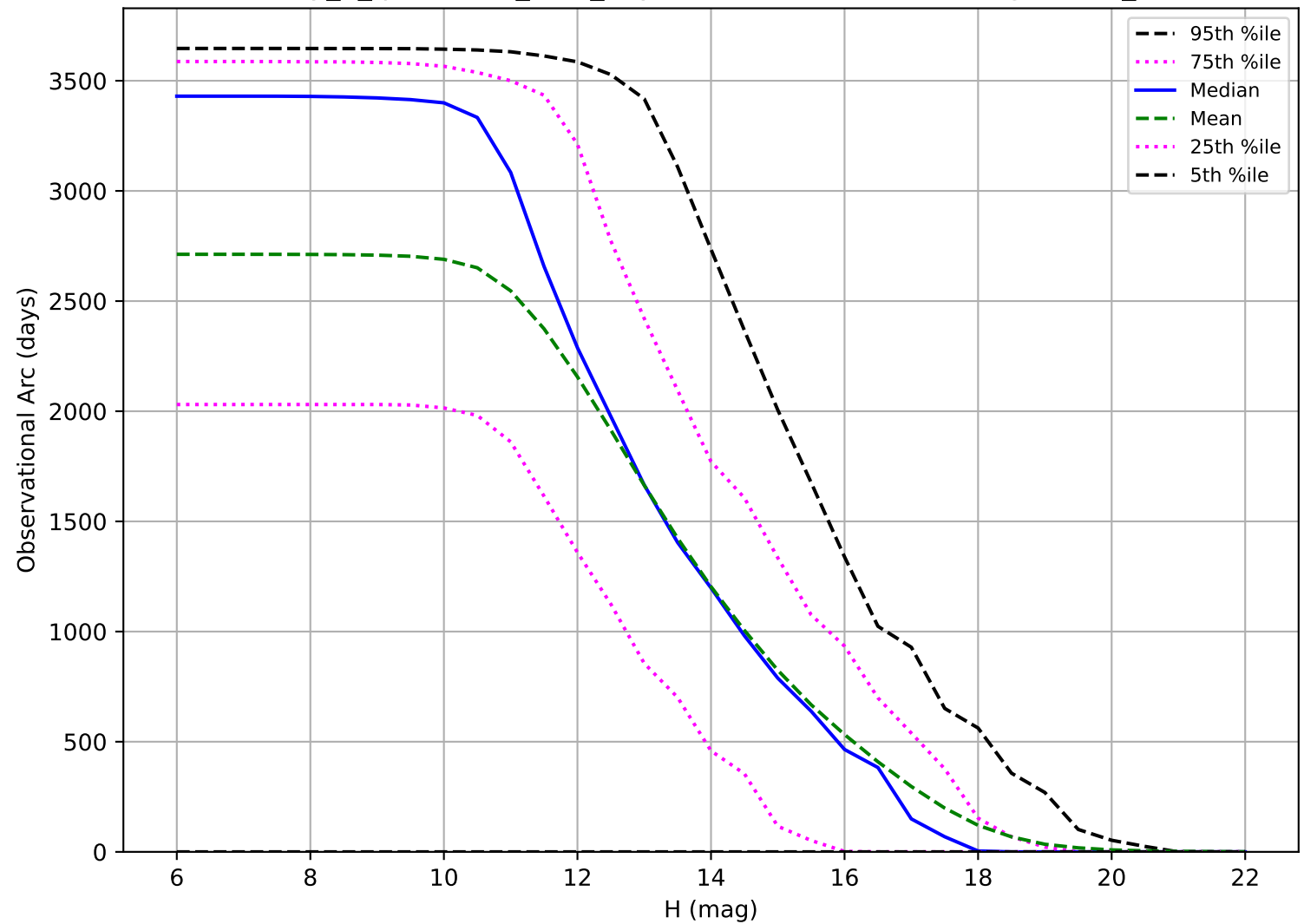
early_u_fpextra3.0_v3.4_10yrs: Observational Arc Length OCC_r5
