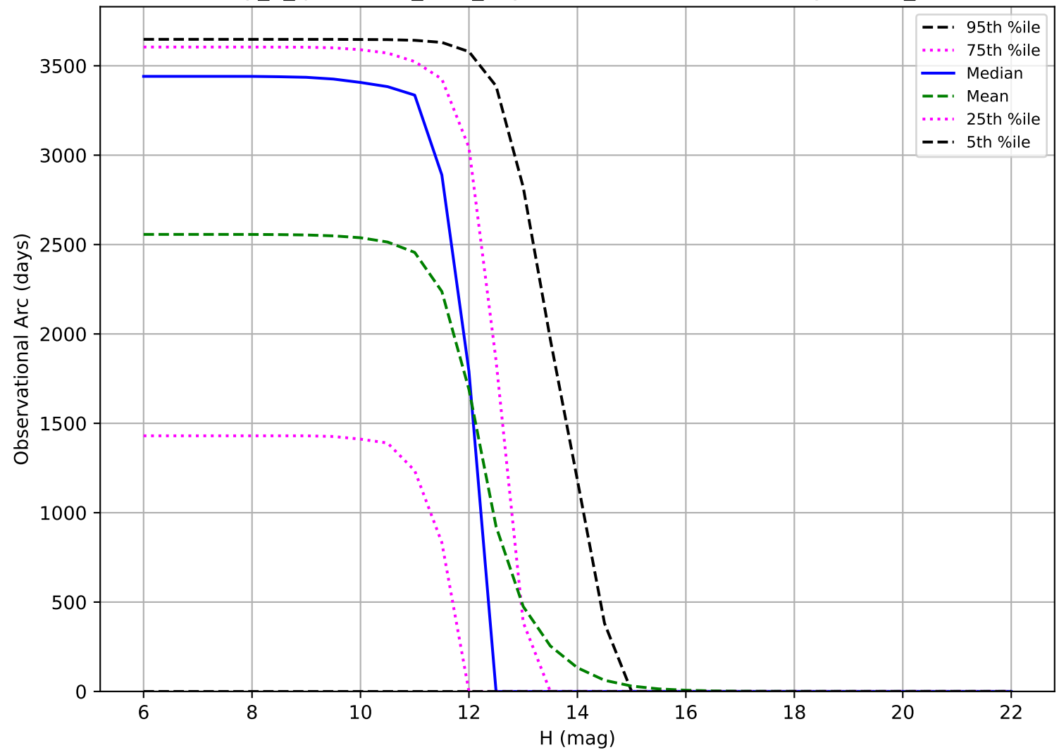
early_u_fpextra3.0_v3.4_10yrs: Observational Arc Length OCC_r20
