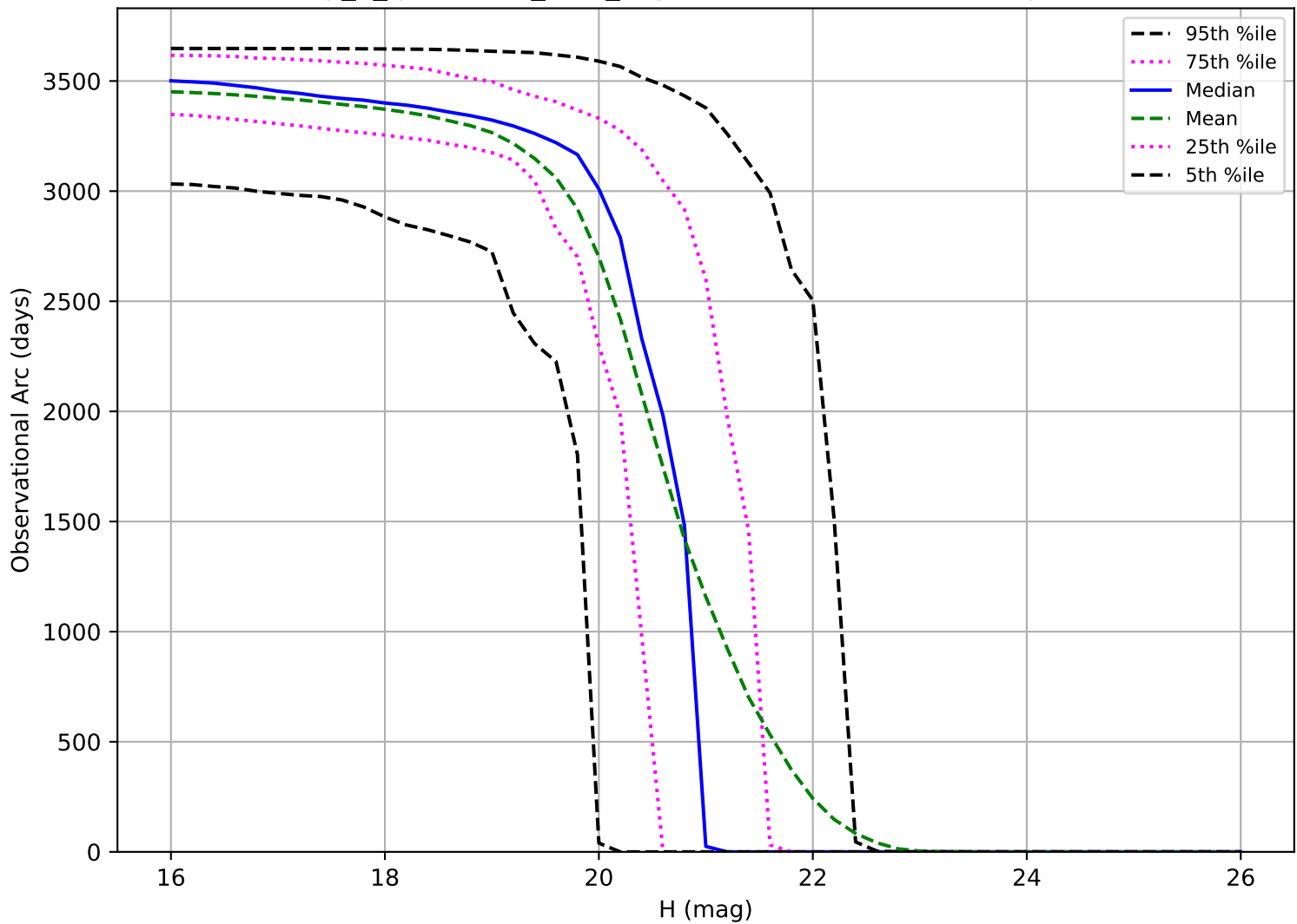
early_u_fpextra3.0_v3.4_10yrs: Observational Arc Length MBA
