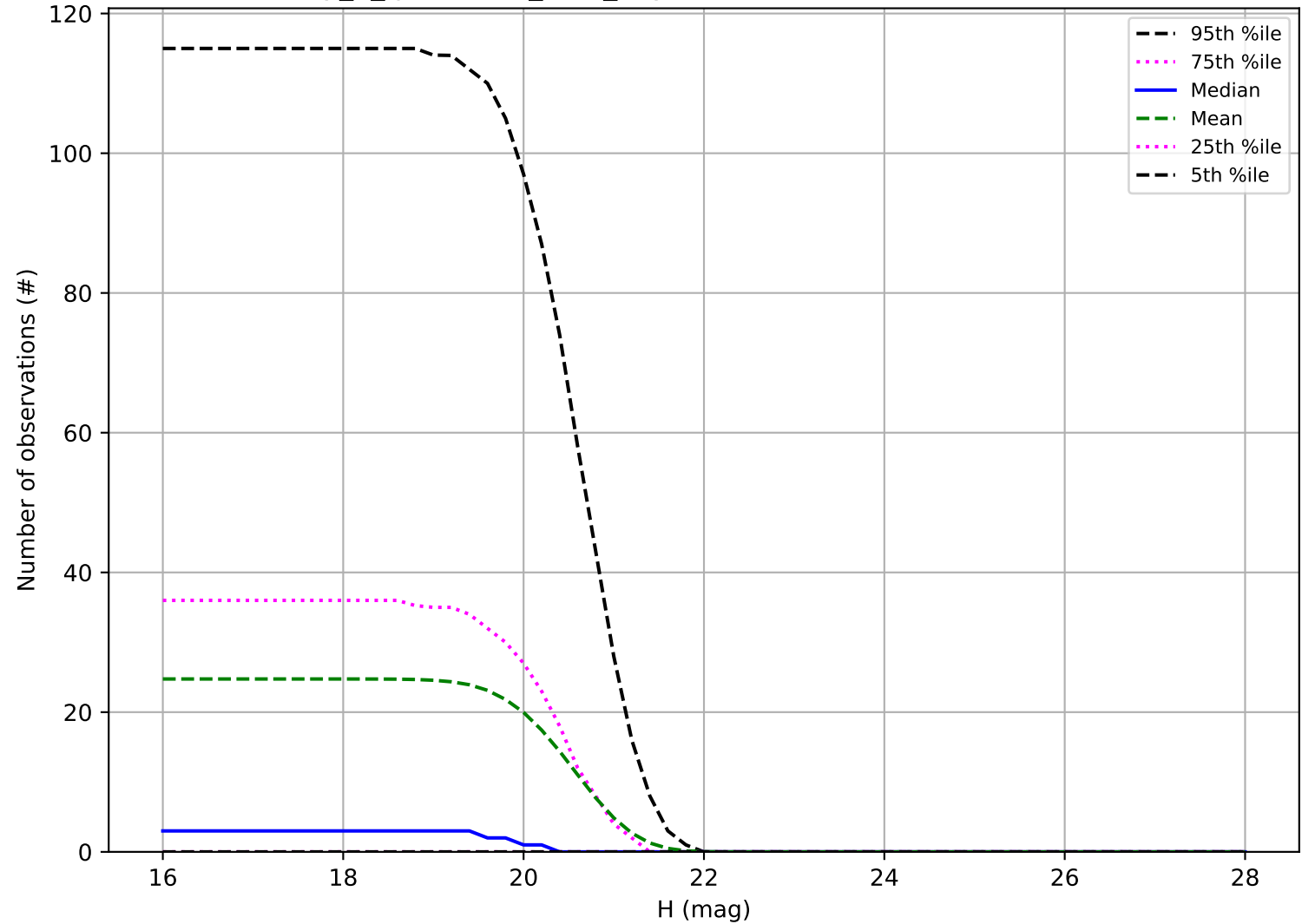
early_u_fpextra3.0_v3.4_10yrs: Number of observations Vatira
