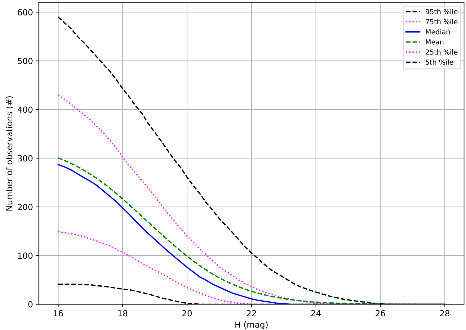
early_u_fpextra3.0_v3.4_10yrs: Number of observations PHA
