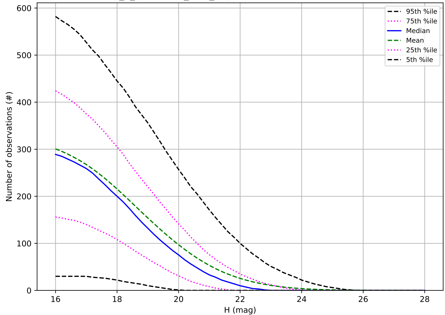
early_u_fpextra3.0_v3.4_10yrs: Number of observations NEO
