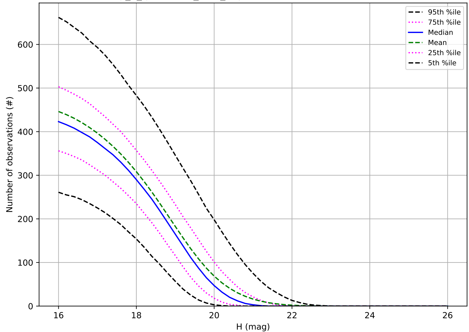
early_u_fpextra3.0_v3.4_10yrs: Number of observations MBA
