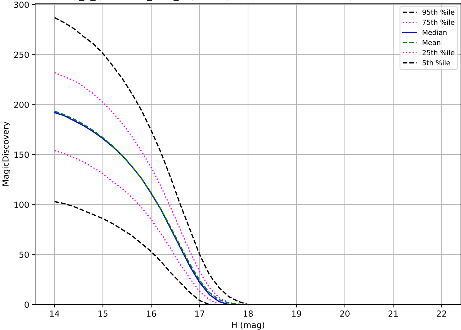
early_u_fpextra3.0_v3.4_10yrs: Trojan 6 detections in 60 nights detection loss
