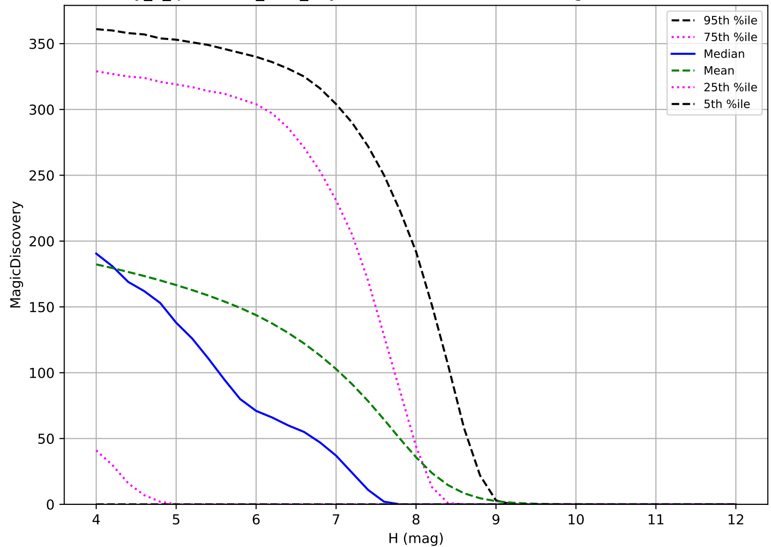
early_u_fpextra3.0_v3.4_10yrs: TNO 6 detections in 60 nights detection loss
