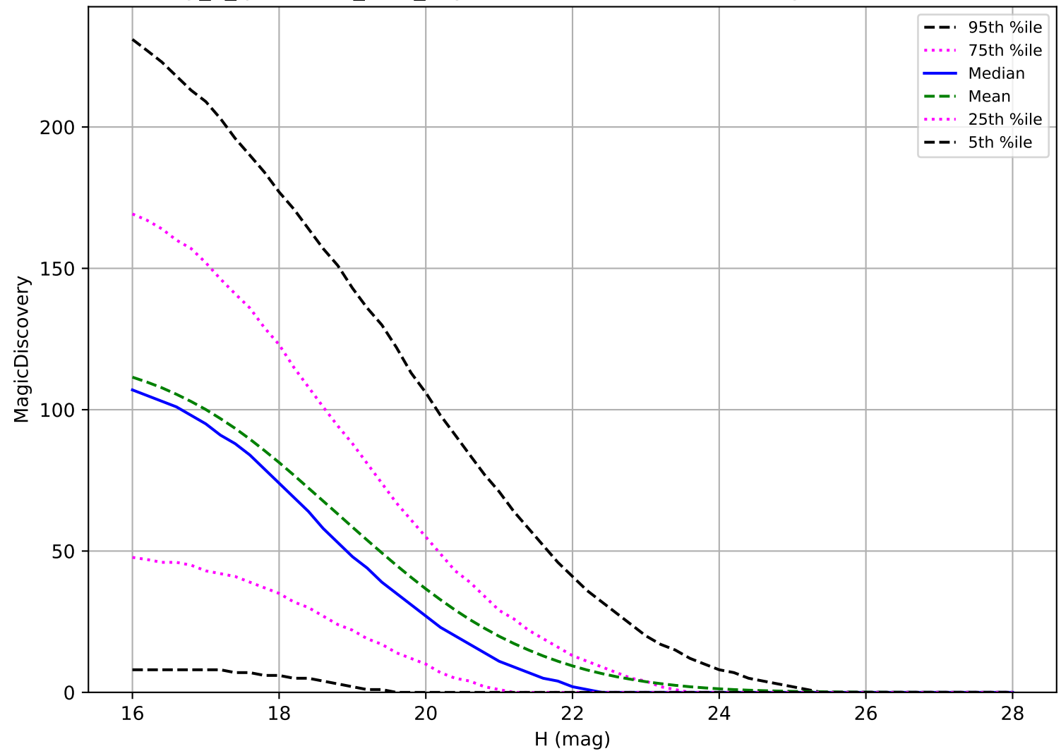
early_u_fpextra3.0_v3.4_10yrs: PHA 6 detections in 60 nights detection loss
