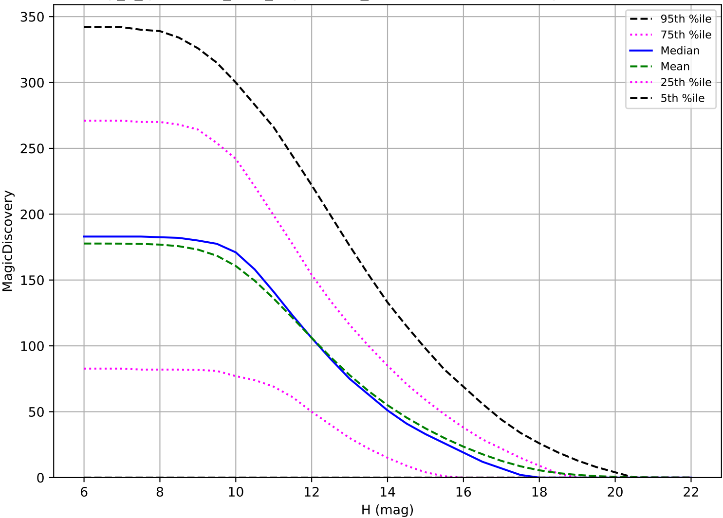
early_u_fpextra3.0_v3.4_10yrs: OCC_r5 6 detections in 60 nights detection loss
