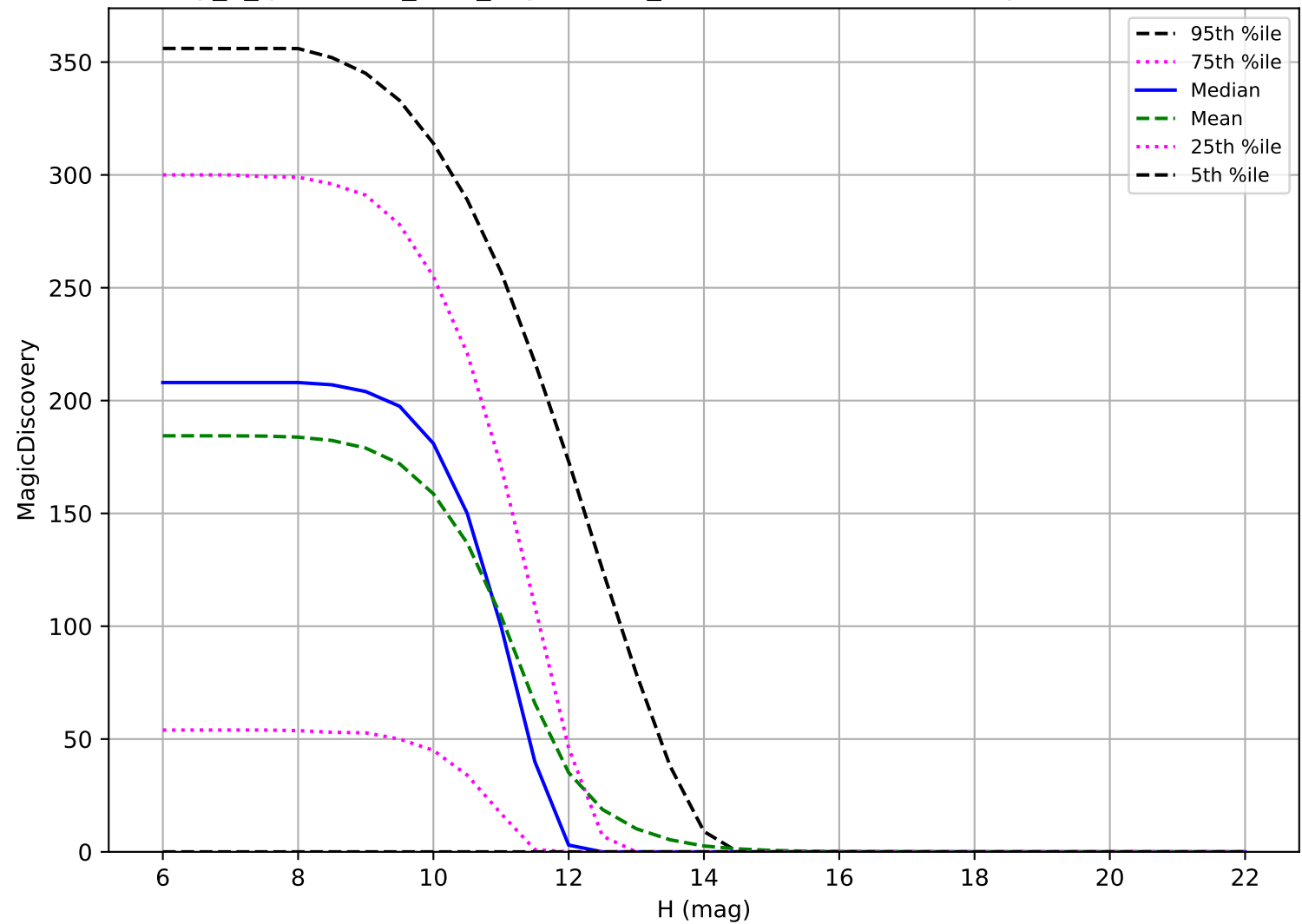
early_u_fpextra3.0_v3.4_10yrs: OCC_r20 6 detections in 60 nights detection loss
