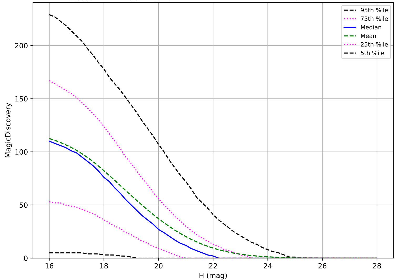
early_u_fpextra3.0_v3.4_10yrs: NEO 6 detections in 60 nights detection loss
