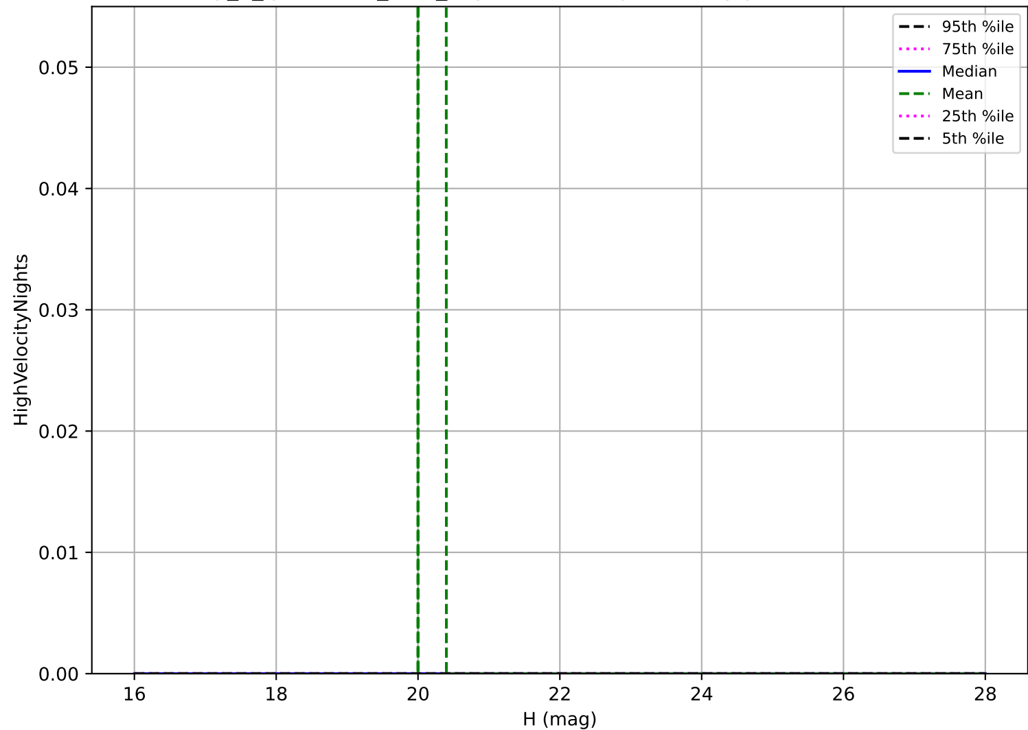
early_u_fpextra3.0_v3.4_10yrs: Vatira High velocity pair detection loss
