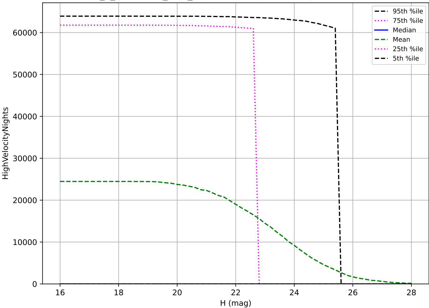
early_u_fpextra3.0_v3.4_10yrs: PHA High velocity pair detection loss
