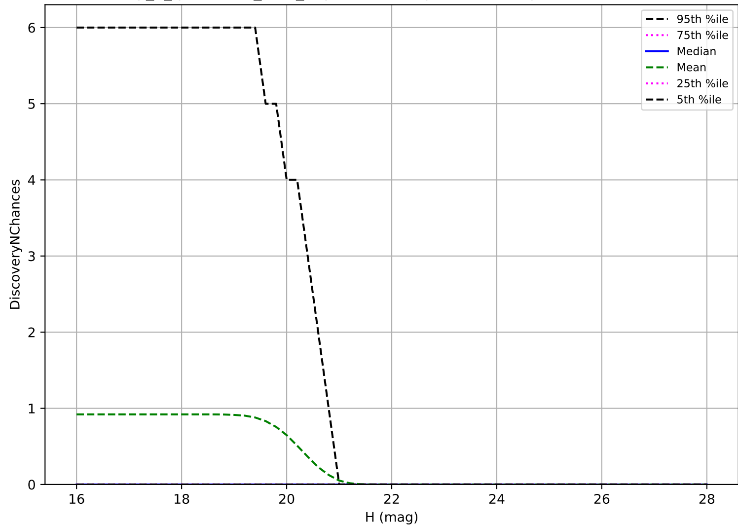
early_u_fpextra3.0_v3.4_10yrs: Vatira 3 pairs in 15 nights detection loss
