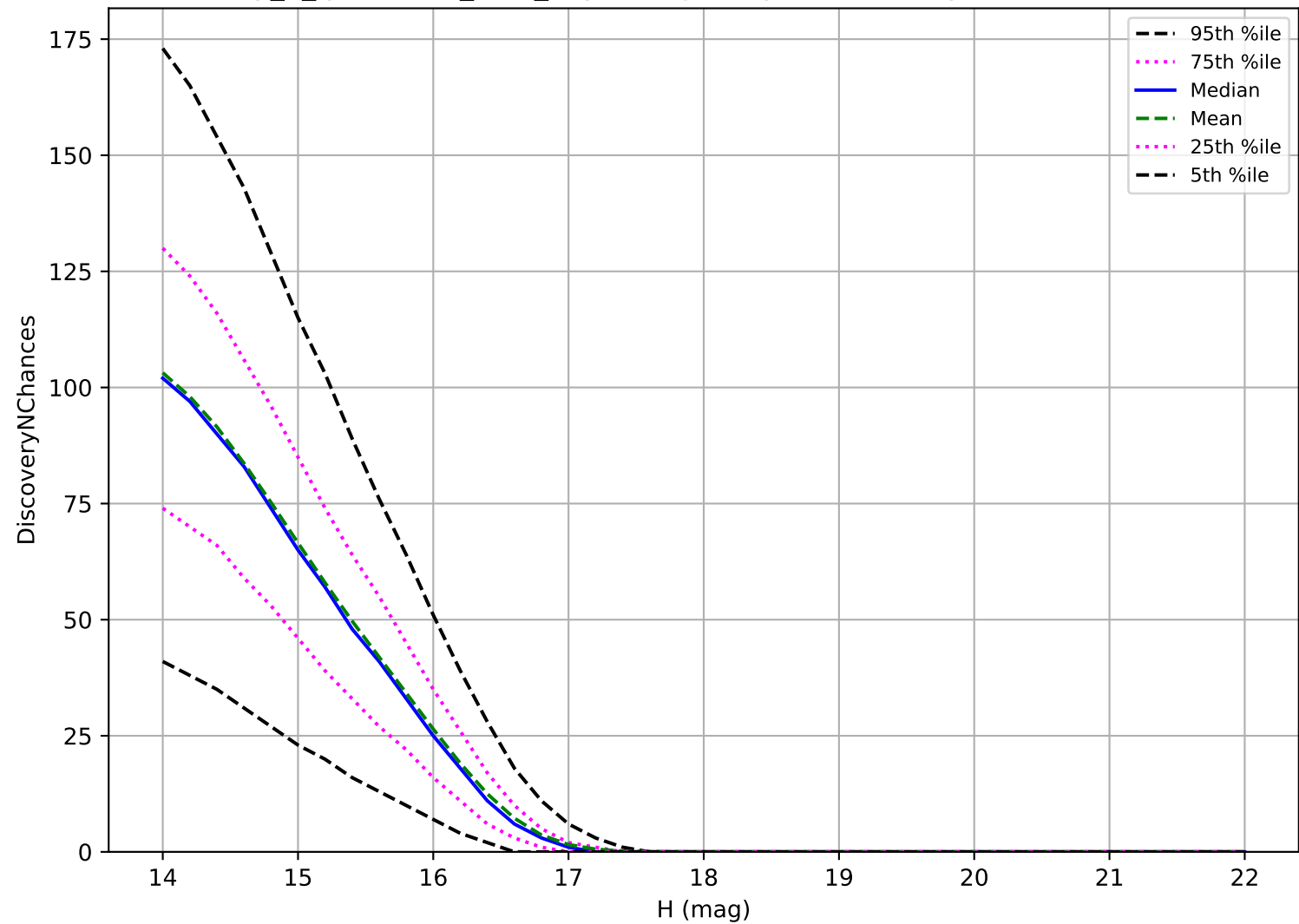
early_u_fpextra3.0_v3.4_10yrs: Trojan 3 pairs in 15 nights detection loss
