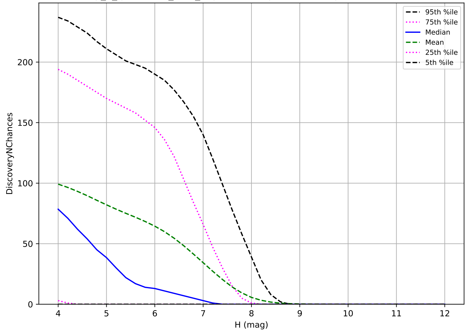
early_u_fpextra3.0_v3.4_10yrs: TNO 3 pairs in 15 nights detection loss
