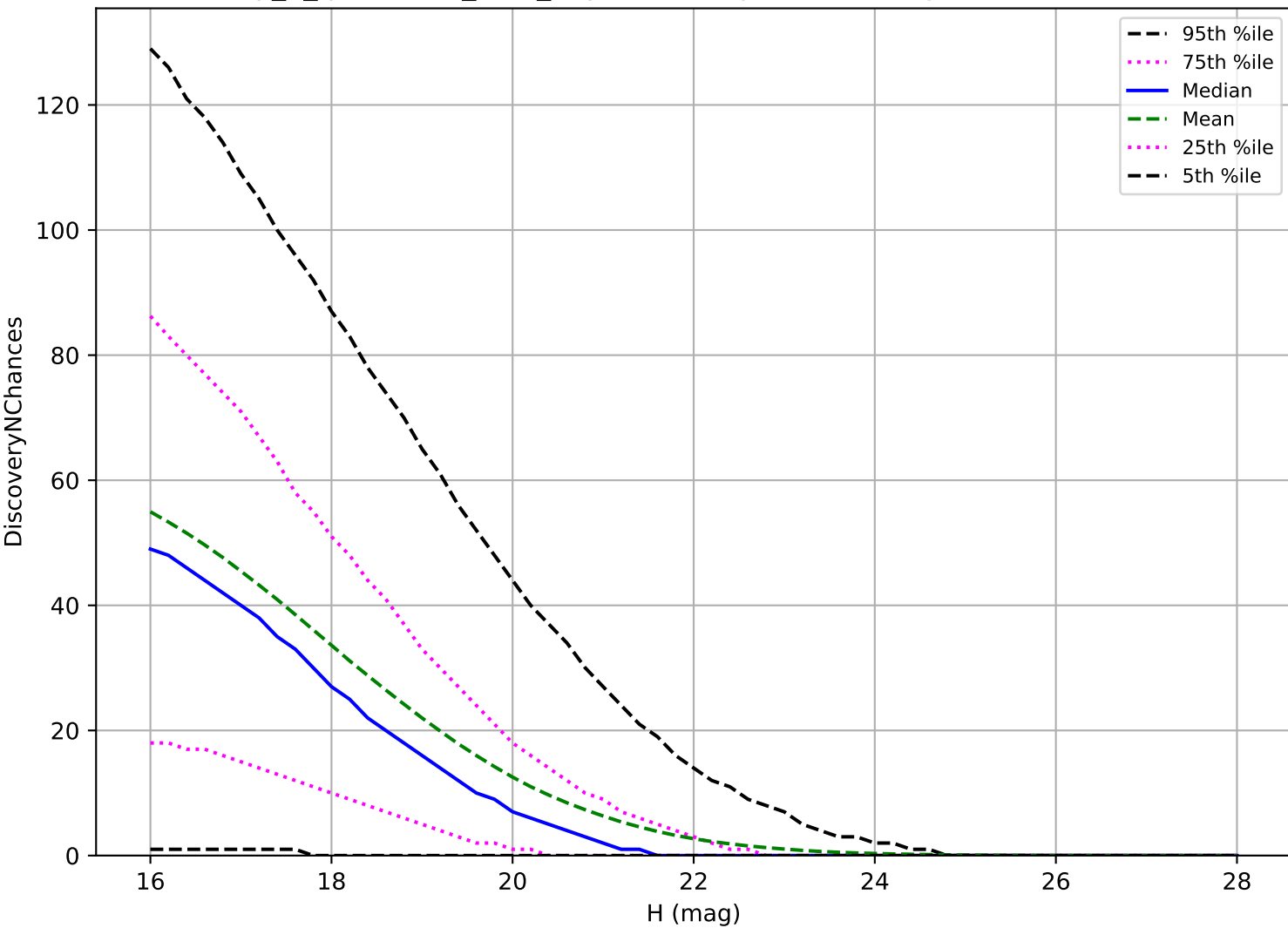
early_u_fpextra3.0_v3.4_10yrs: PHA 3 pairs in 15 nights detection loss
