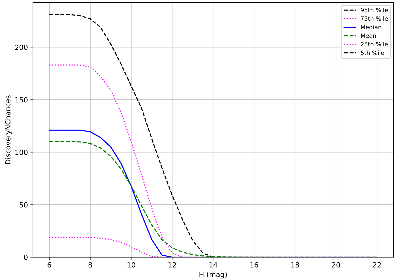
early_u_fpextra3.0_v3.4_10yrs: OCC_r20 3 pairs in 15 nights detection loss
