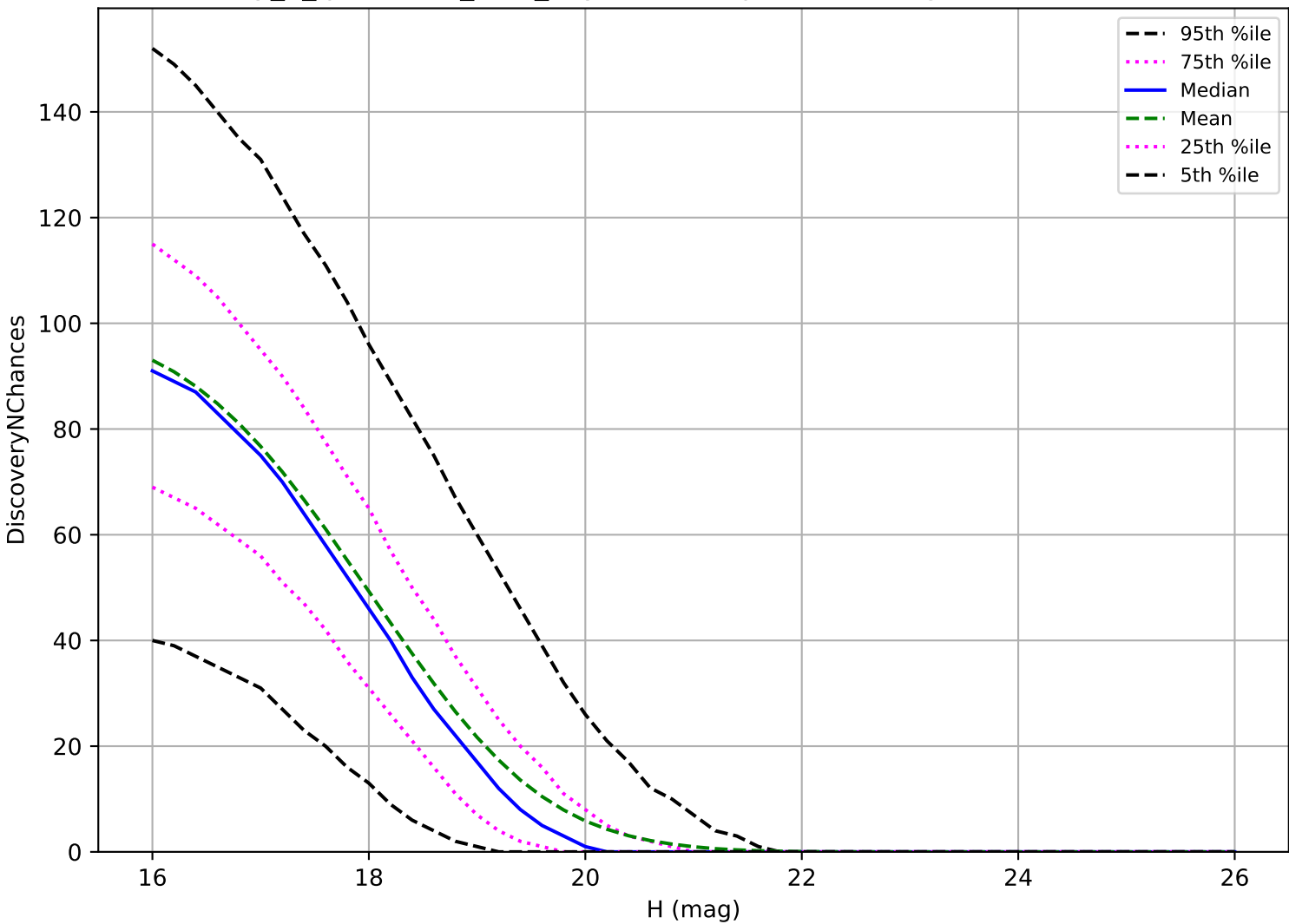
early_u_fpextra3.0_v3.4_10yrs: MBA 3 pairs in 15 nights detection loss
