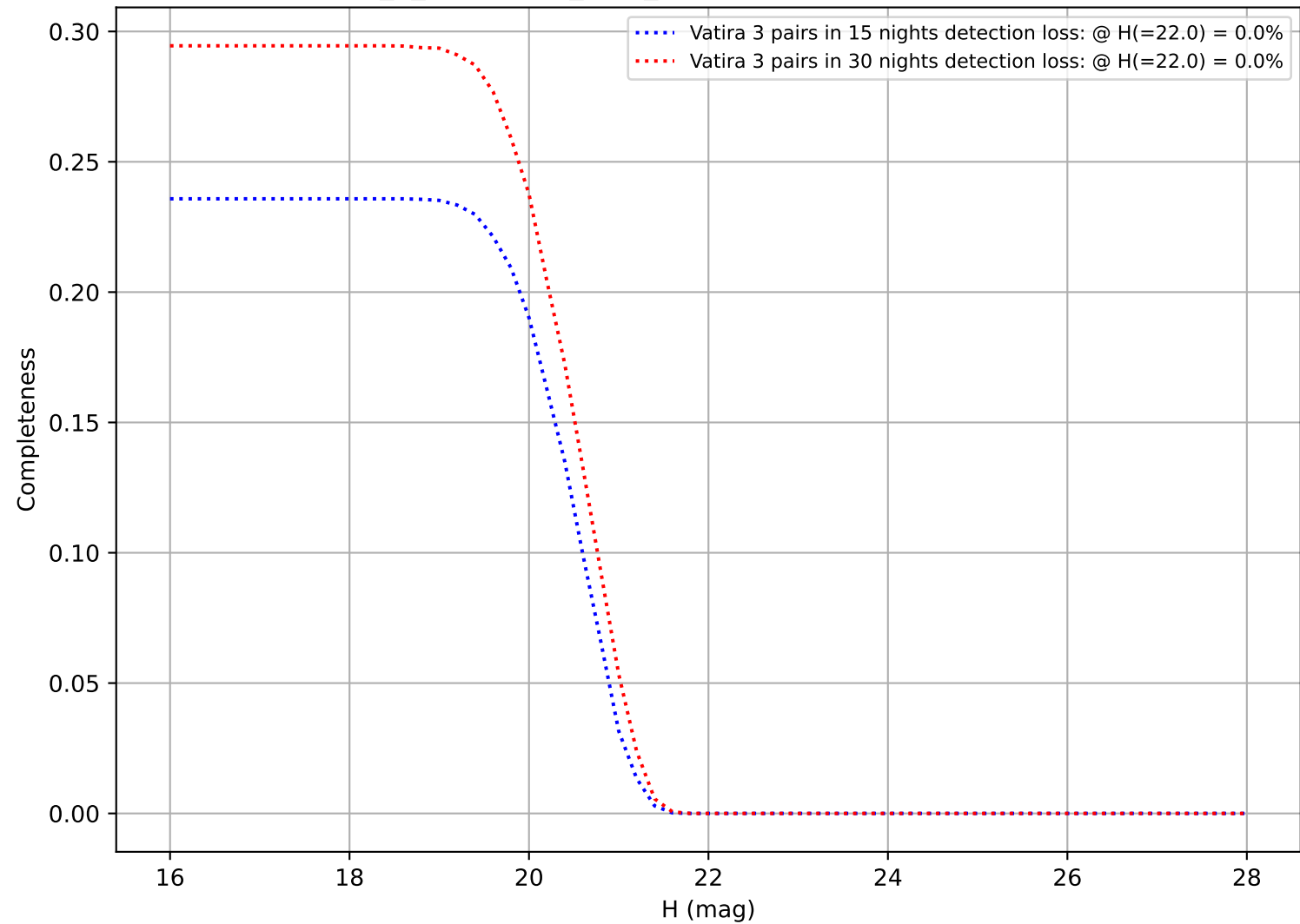
early_u_fpextra3.0_v3.4_10yrs: DifferentialCompleteness
