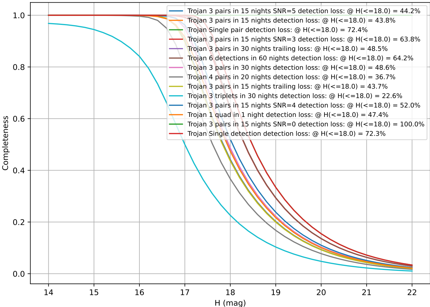
early_u_fpextra3.0_v3.4_10yrs: CumulativeCompleteness
