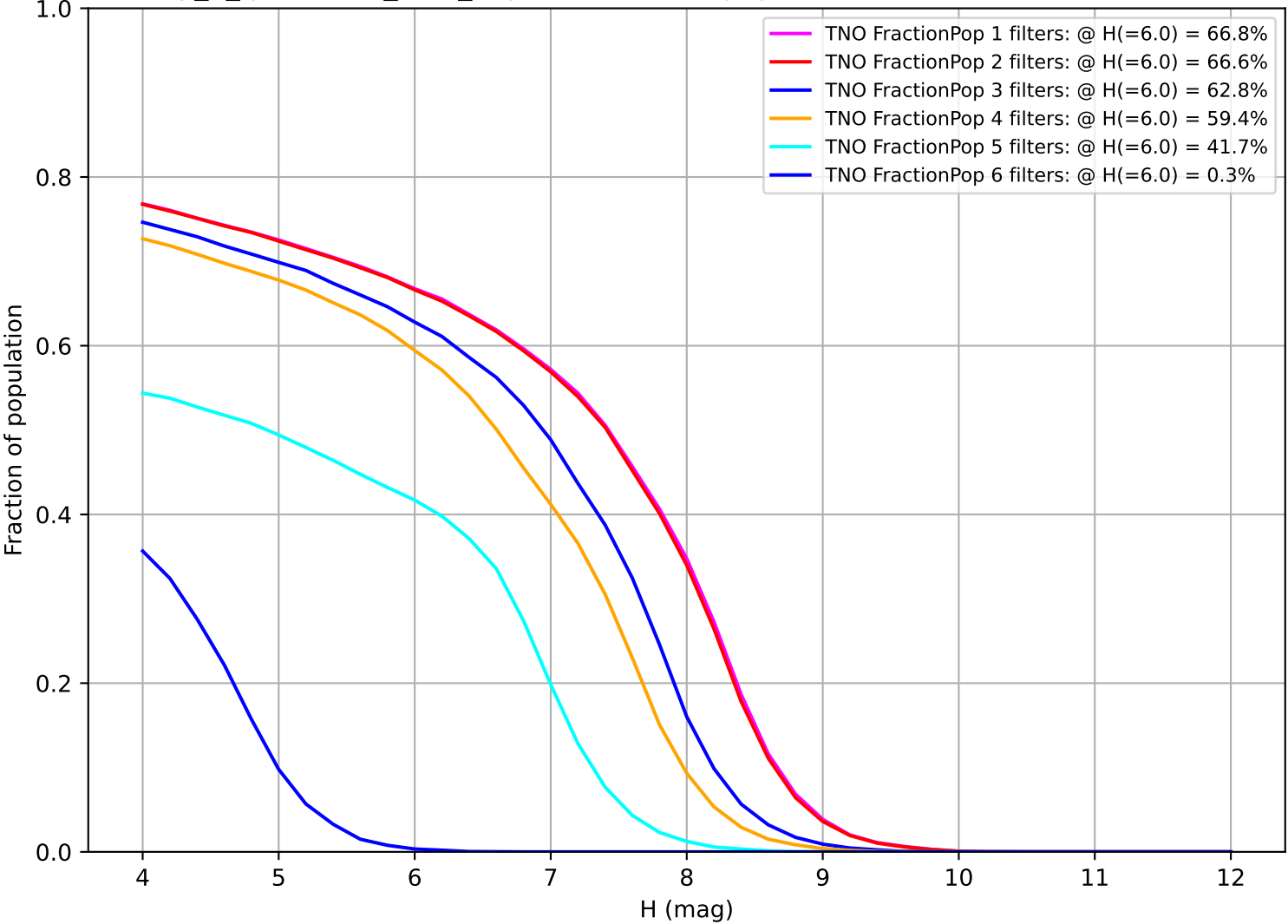
early_u_fpextra3.0_v3.4_10yrs: Fraction of population with colors in X filters TNO
