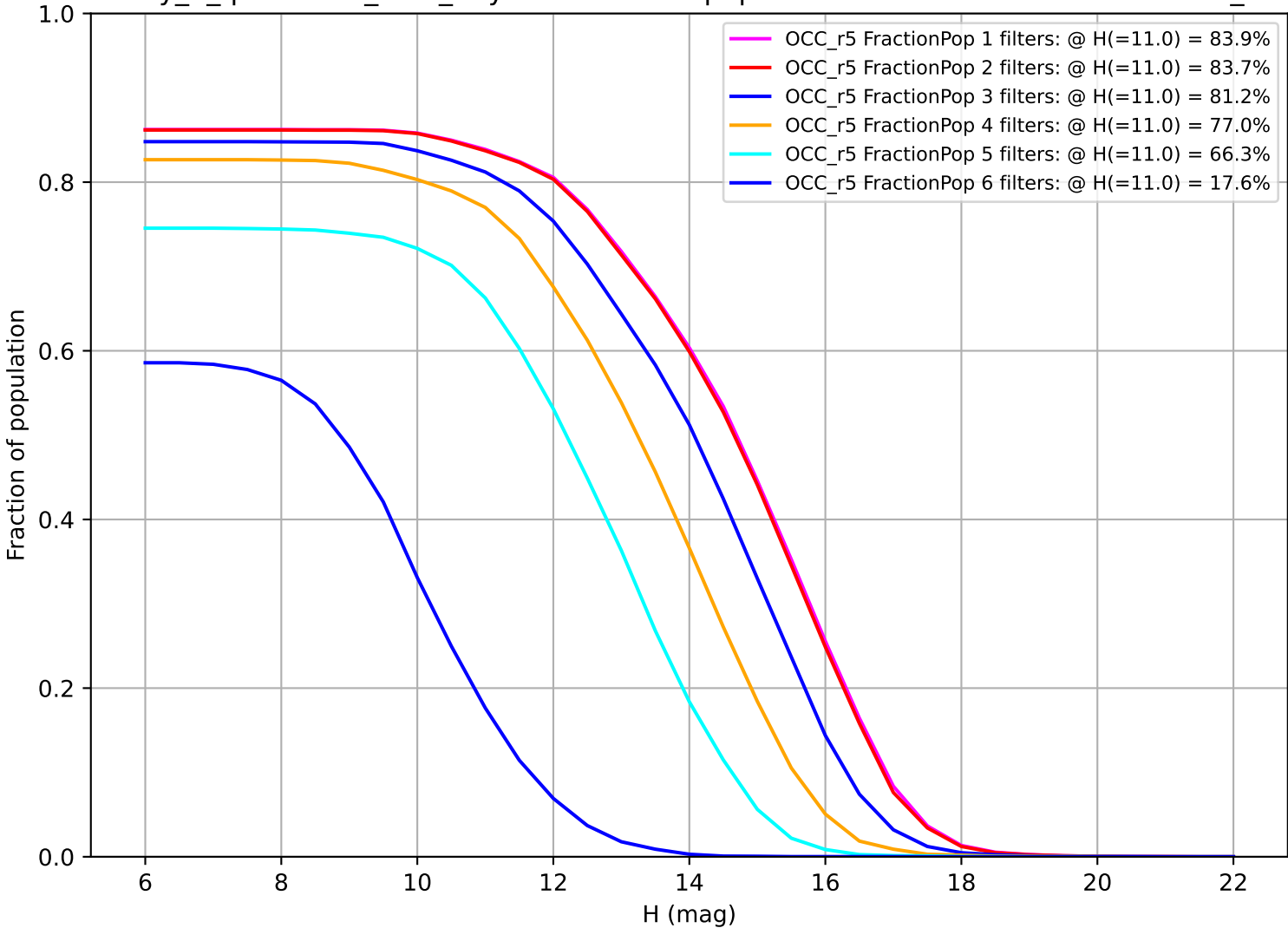
early_u_fpextra3.0_v3.4_10yrs: Fraction of population with colors in X filters OCC_r5
