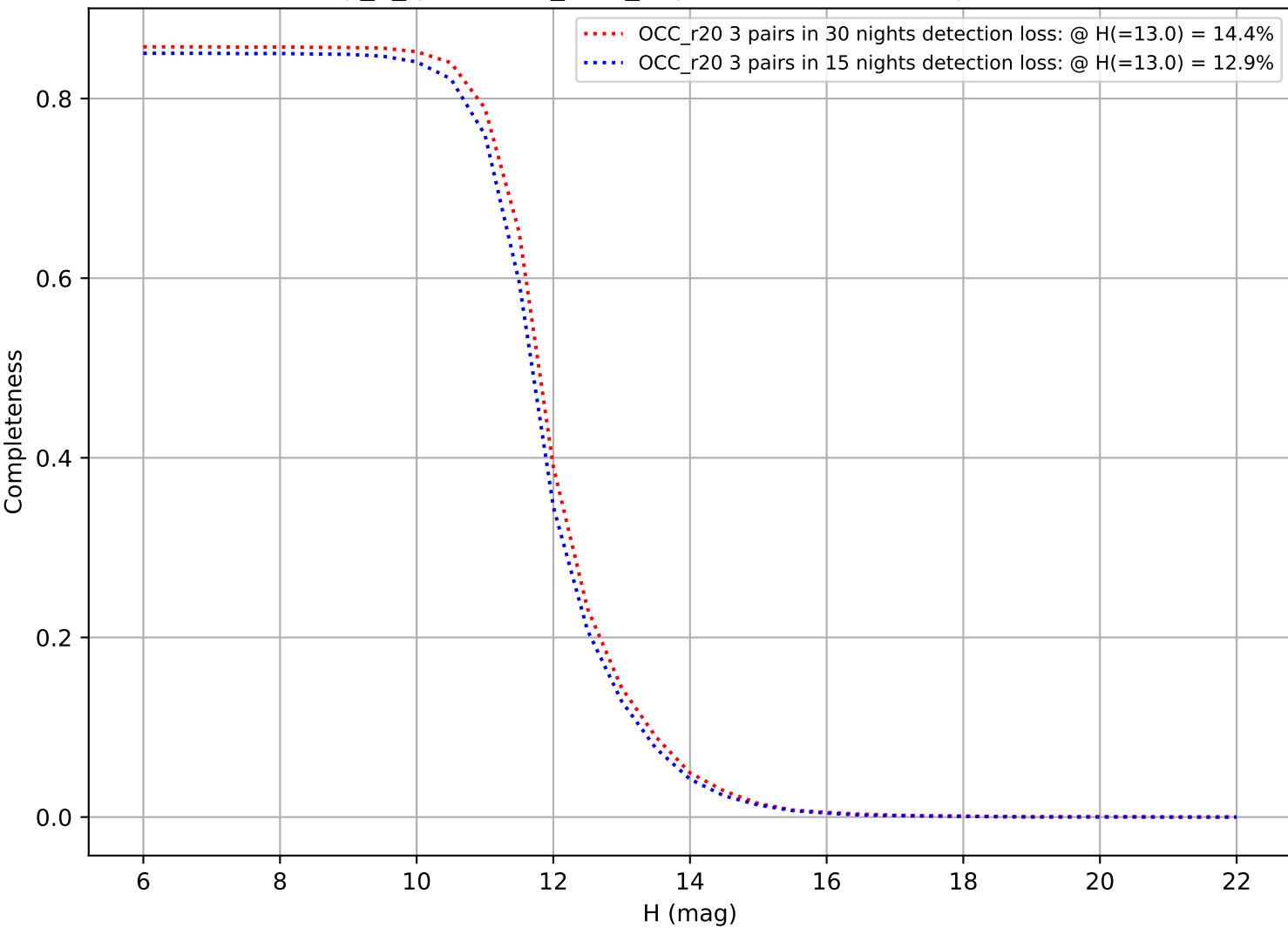
early_u_fpextra3.0_v3.4_10yrs: DifferentialCompleteness
