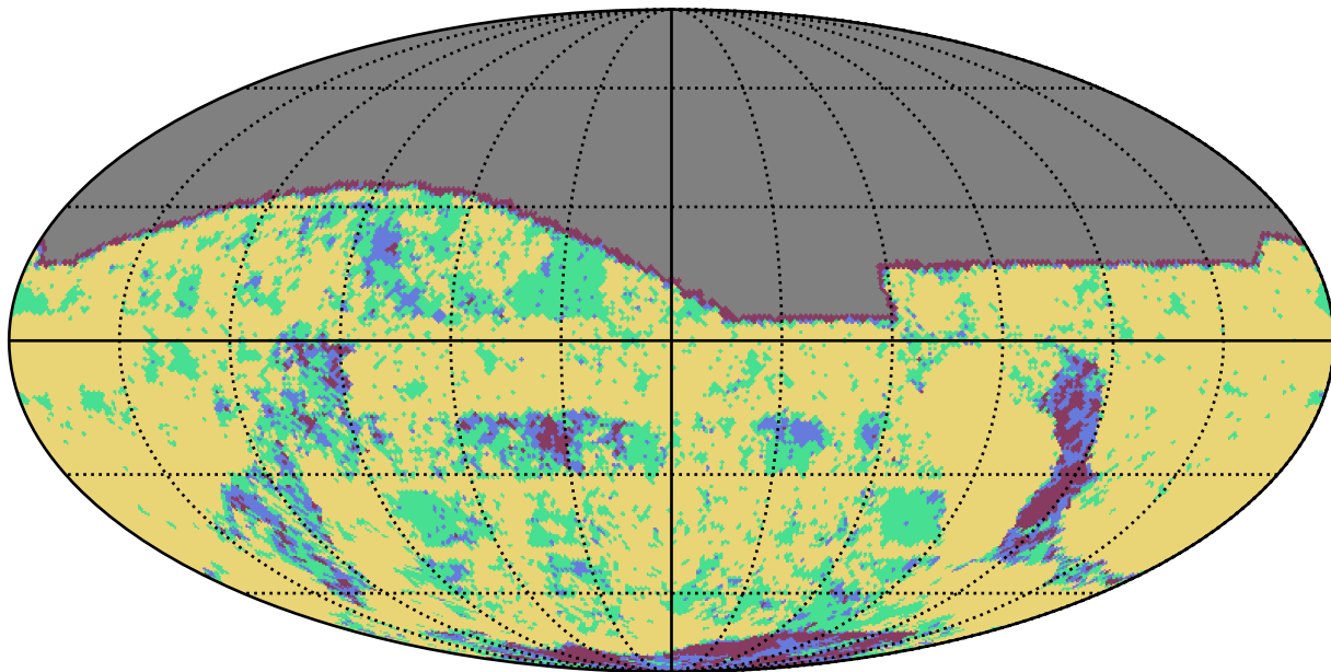
early_u_fpextra3.0_v3.4_10yrs g band: YearCoverage night
