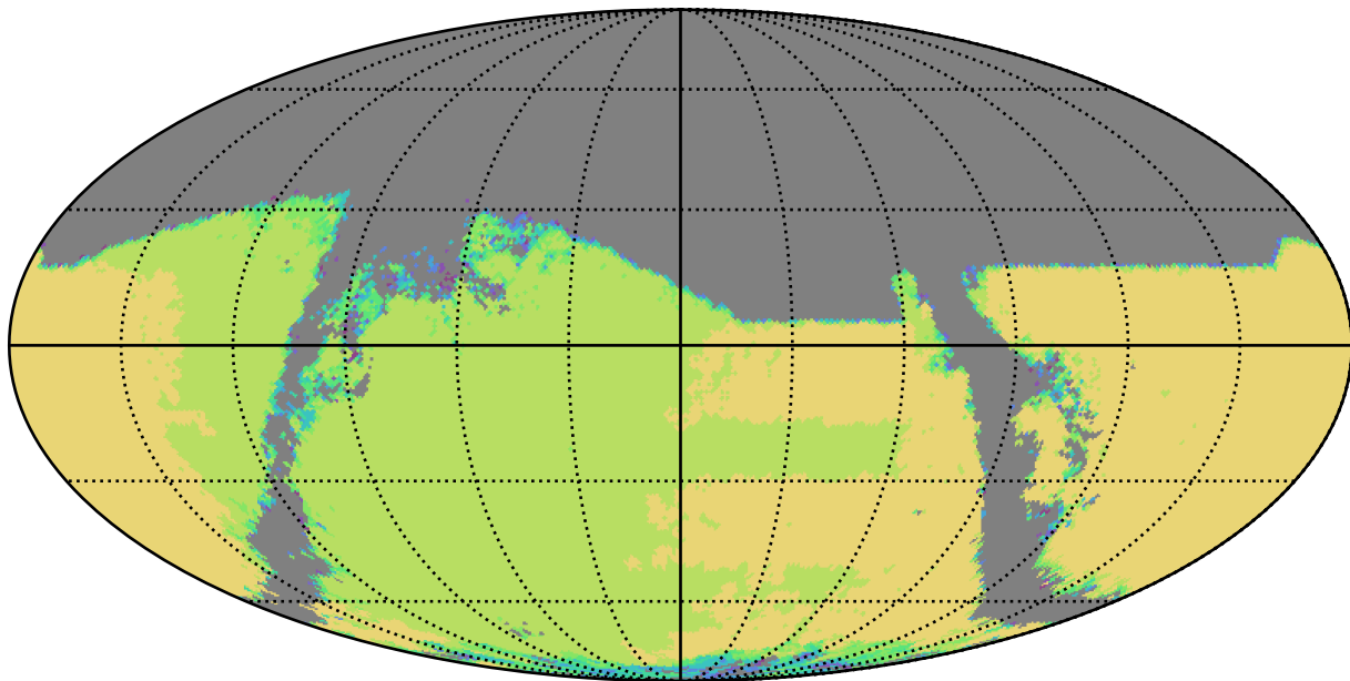
early_u_fpextra3.0_v3.4_10yrs : TDC_campaign
