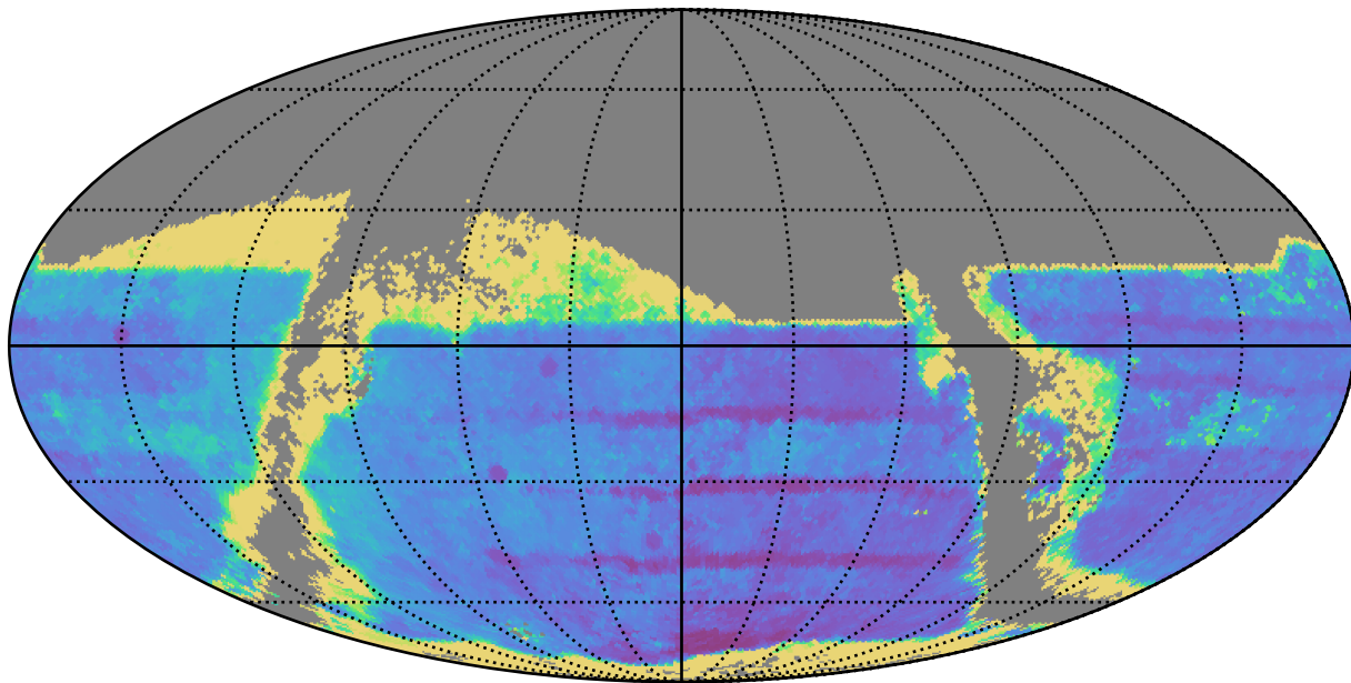
early_u_fpextra3.0_v3.4_10yrs : TDC_accuracy
