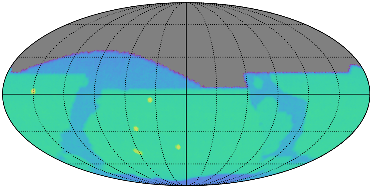
early_u_fpextra3.0_v3.4_10yrs z: SurfaceBrightLimit
