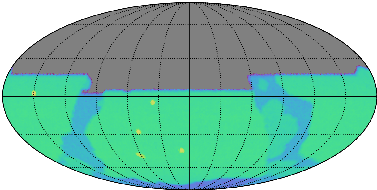
early_u_fpextra3.0_v3.4_10yrs y: SurfaceBrightLimit
