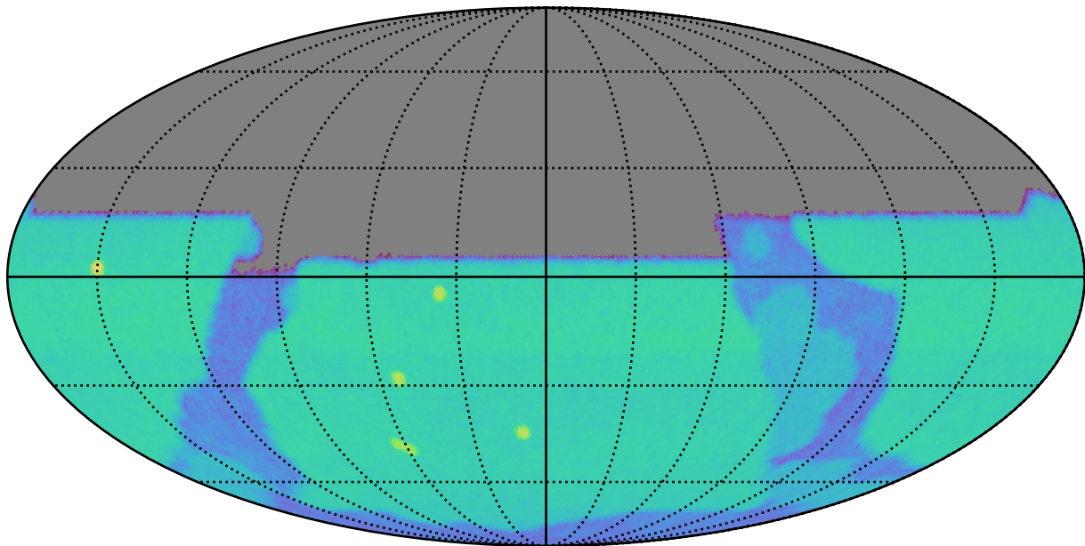
early_u_fpextra3.0_v3.4_10yrs u: SurfaceBrightLimit
