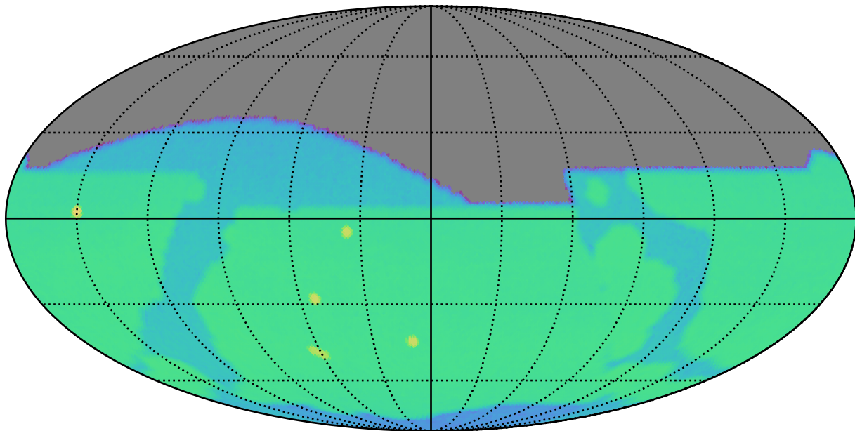
early_u_fpextra3.0_v3.4_10yrs r: SurfaceBrightLimit
